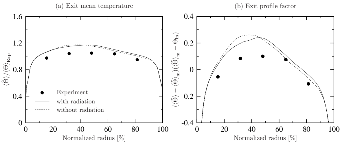
Figure 16. Azimuthally averaged statistics at combustor exit plane: (a) normalized temperature and (b) temperature profile factor.
