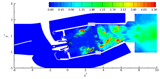
(b) Instantaneous Favre-filtered NO mole fraction (normalized)
